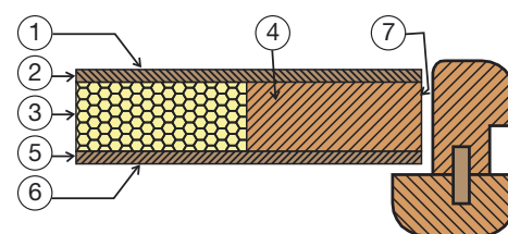
JB DOOR SANDWICH CONSTRUCTION:
